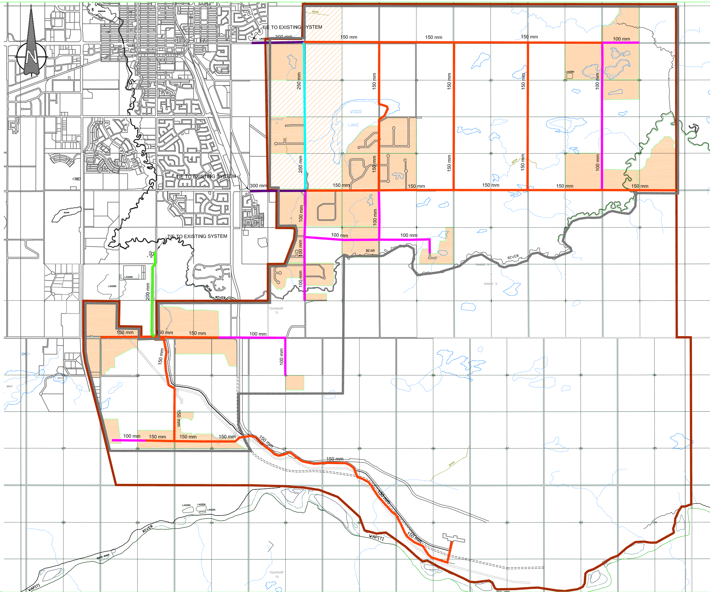
Figure 6.3.1.2 SOUTH EAST AREA SERVICING STUDY TRICKLE WATER SYSTEM WITH FIRE FLOW FOR UR LAND USE AREA ONLY CONCEPT PLAN ISL Infrastructure Systems Ltd.
