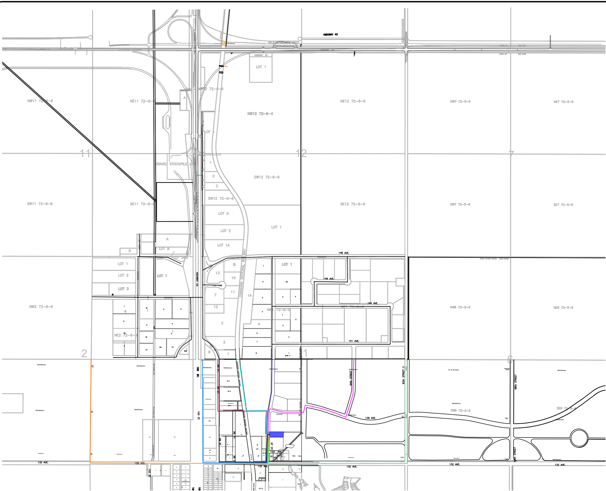
Figure 3.1 COUNTY OF GRANDE PRAIRIE NORTH COUNTY INDUSTRIAL SUBDIVISION WATER DISTRIBUTION SYSTEM MASTER PLAN REGIONAL WATER TRANSMISSION LINE OPTIONS
