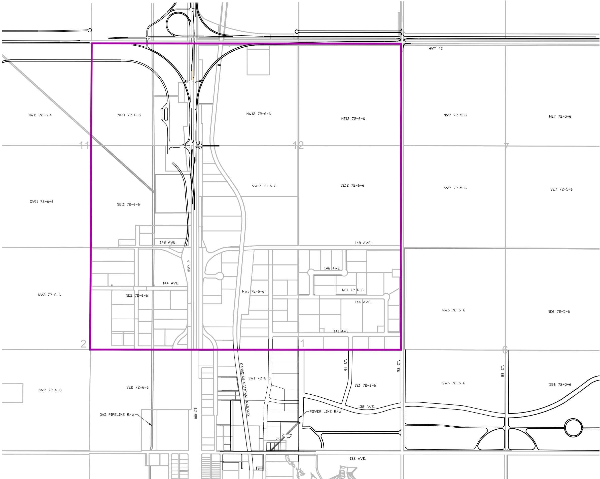
Figure 1.1 COUNTY OF GRANDE PRAIRIE NORTH COUNTY INDUSTRIAL SUBDIVISION WATER DISTRIBUTION SYSTEM MASTER PLAN STUDY AREA
