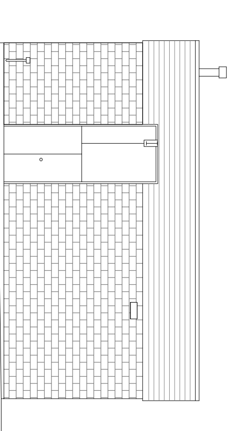
LIFT STATION - FRONT VIEW ELEVATION SCALE 1:50
