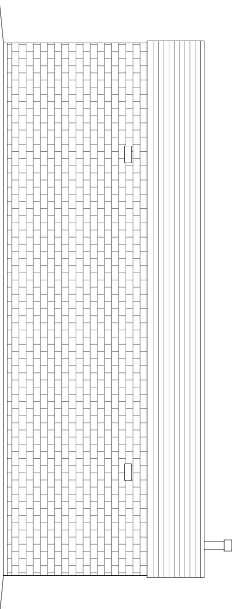
LIFT STATION - FRONT VIEW ELEVATION SCALE 1:50
