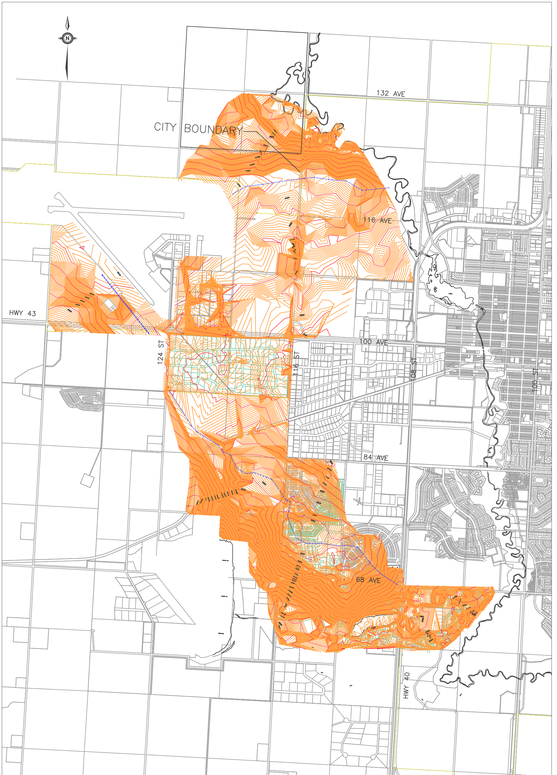
AQUATERA UTILITIES INC 116th STREET SANITARY TRUNK EXPANDED SYSTEM CONTOUR PLAN FIGURE 4
